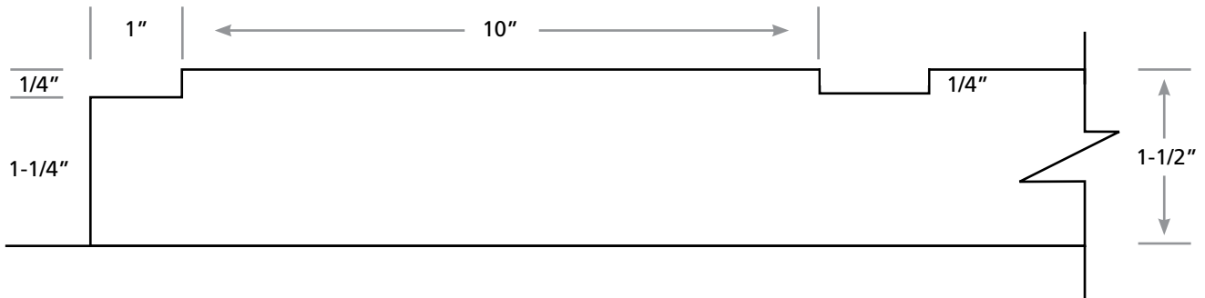
1/4" deep x 1-1/2" wide (10" on center)
